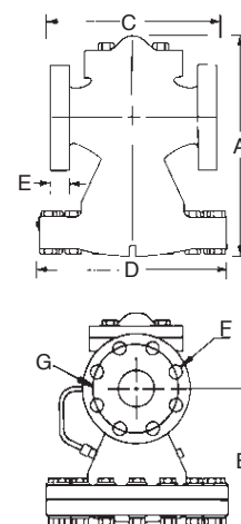
Model 2200 & 2250 Flanged Ends
