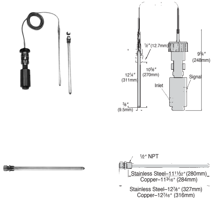
Well for Series STPA
