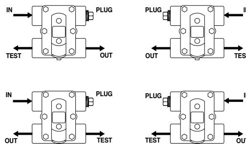
Series H Piping Options
