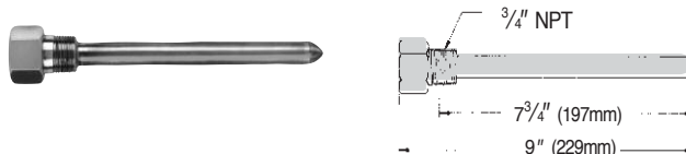
Well for Series 315 PNT
